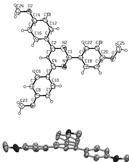
Figure 1. Molecular structure of compound 1 with the atomic labelling scheme. Selected bond lengths [Å]: C(1)–C(17) 1.483, C(2)–C(11) 1.501, C(1)–C(5) 1.479, C(1)–N(2) 1.355, N(2)–C(2) 1.361, C(2)–C(3) 1.314, C(3)–C(4) 1.332, C(4)–N(1) 1.400, N(1)–C(1) 1.364.
