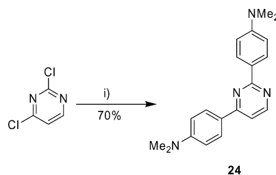
Scheme 10. Reagents and conditions: i) p\text{-Me}_2\text{NC}_6\text{H}_4\text{B}(\text{OH})_2 , [\text{Pd}(\text{PPh}_3)_4] , \text{Cs}_2\text{CO}_3 , toluene, \text{H}_2\text{O} , \Delta , 40 h.
