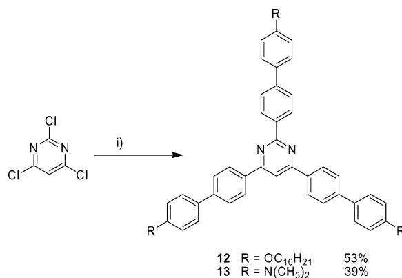
Scheme 5. Reagents and conditions: i) p - \text{RC}_6\text{H}_4\text{C}_6\text{H}_4\text{B}(\text{OH})_2 , [\text{Pd}(\text{PPh}_3)_4] , \text{Cs}_2\text{CO}_3 , toluene, \text{H}_2\text{O} , \Delta , 40 h.
