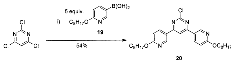
Scheme 8. Reagents and conditions: i) [\text{Pd}(\text{PPh}_3)_2\text{Cl}_2] , dioxane, \text{Na}_2\text{CO}_3 , \Delta , 8 h.
