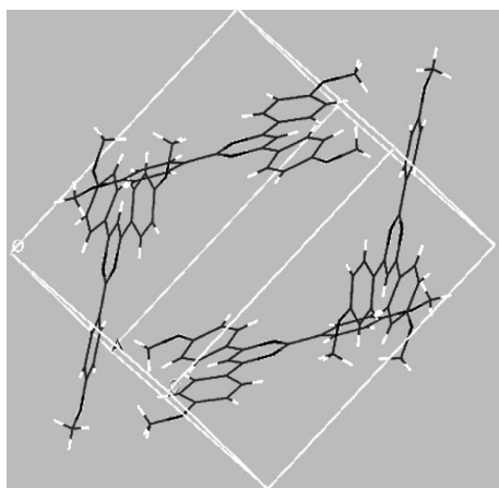
Figure 2. Crystal structure of 1 .
