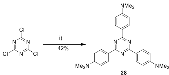
Scheme 13. Reagents and conditions: i) p -Me 2 NC 6 H 4 B(OH) 2 , [Pd(PPh 3 ) 4 ], Cs 2 CO 3 , toluene, H 2 O, Δ, 24 h.
