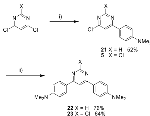
Scheme 9. Reagents and conditions: i) p\text{-Me}_2\text{NC}_6\text{H}_4\text{B}(\text{OH})_2 , [\text{Pd}(\text{PPh}_3)_4] , \text{Cs}_2\text{CO}_3 , toluene, \text{H}_2\text{O} , \Delta , 24 h; ii) p\text{-Me}_2\text{NC}_6\text{H}_4\text{B}(\text{OH})_2 , [\text{Pd}(\text{PPh}_3)_4] , \text{Cs}_2\text{CO}_3 , toluene, \text{H}_2\text{O} , \Delta , 48 h.
