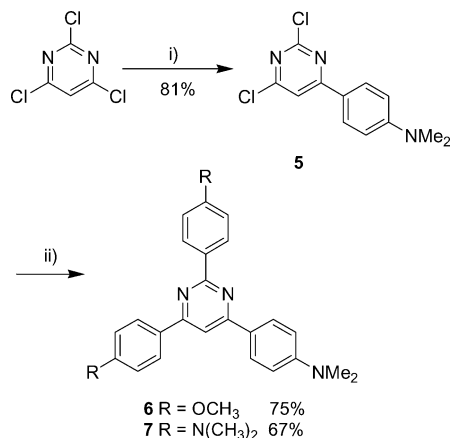
Scheme 2. Reagents and conditions: i) p -( \text{Me}_2\text{N} ) \text{C}_6\text{H}_4\text{B}(\text{OH})_2 , [\text{Pd}(\text{PPh}_3)_4] , \text{Cs}_2\text{CO}_3 , toluene, \text{H}_2\text{O} , \Delta , 40 h; ii) p - \text{RC}_6\text{H}_4\text{B}(\text{OH})_2 , [\text{Pd}(\text{PPh}_3)_4] , \text{Cs}_2\text{CO}_3 , toluene, \text{H}_2\text{O} , \Delta , 40 h.
