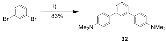
Scheme 15. Reagents and conditions: i) p -Me 2 NC 6 H 4 B(OH) 2 , [Pd(PPh 3 ) 4 ], Cs 2 CO 3 , toluene, H 2 O, Δ, 24 h.
