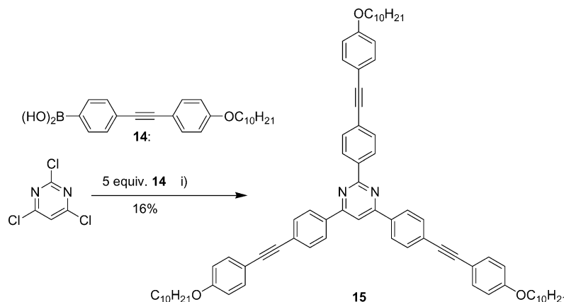
Scheme 6. Reagents and conditions: i) [\text{Pd}(\text{PPh}_3)_4] , \text{Cs}_2\text{CO}_3 , toluene, \text{H}_2\text{O} , \Delta , 40 h.
