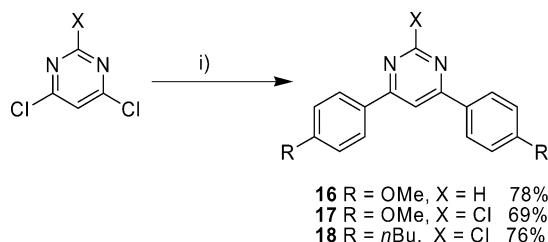
Scheme 7. Reagents and conditions: p\text{-RC}_6\text{H}_4\text{B}(\text{OH})_2 , [\text{Pd}(\text{PPh}_3)_4] , \text{Cs}_2\text{CO}_3 , toluene, \text{H}_2\text{O} , \Delta , 40 h.
