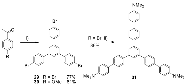
Scheme 14. Reagents and conditions: i) SiCl 4 , EtOH, room temp., 15 h; ii) p -Me 2 NC 6 H 4 B(OH) 2 , [Pd(PPh 3 ) 4 ], Cs 2 CO 3 , toluene, H 2 O, Δ, 24 h.
