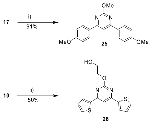
Scheme 11. Reagents and conditions: i) MeONa/MeOH, 60 °C, 24 h; ii) HOCH 2 CH 2 ONa/HOCH 2 CH 2 OH, 15 h, room temp.
