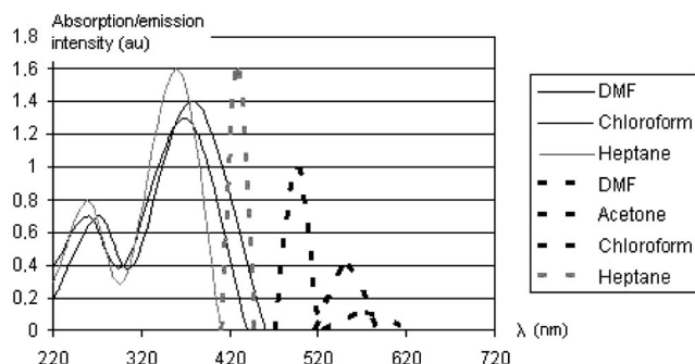
Figure 3. Normalised absorbance and emission (dotted line) spectra of compound 13 in various solvents.
