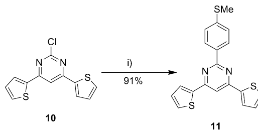
Scheme 4. Reagents and conditions: i) p - \text{MeSC}_6\text{H}_4\text{B}(\text{OH})_2 , [\text{Pd}(\text{PPh}_3)_4] , \text{Cs}_2\text{CO}_3 , toluene, \text{H}_2\text{O} , \Delta , 40 h.
