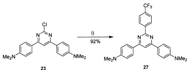
Scheme 12. Reagents and conditions: i) p -F 3 CC 6 H 4 B(OH) 2 , [Pd(PPh 3 ) 4 ], Cs 2 CO 3 , toluene, H 2 O, Δ, 40 h.
