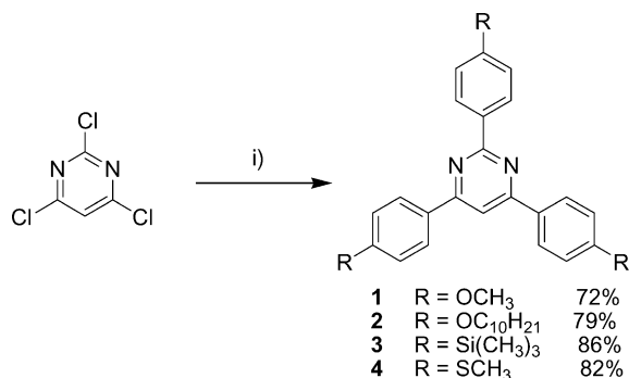
Scheme 1. Reagents and conditions: i) p - \text{RC}_6\text{H}_4\text{B}(\text{OH})_2 , [\text{Pd}(\text{PPh}_3)_4] , \text{Cs}_2\text{CO}_3 , toluene, \text{H}_2\text{O} , \Delta , 40 h.
