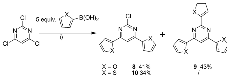
Scheme 3. Reagents and conditions: i) [\text{Pd}(\text{PPh}_3)_4] , \text{Cs}_2\text{CO}_3 , toluene, \text{H}_2\text{O} , \Delta , 40 h.
